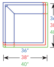
Cube Wedge 5506CP, 36" 6606CP, 38" 7706CP, 40"
