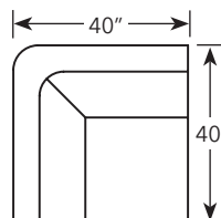
13986CP Cube Wedge 40" x 40"
