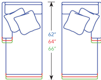
Left Facing Chaise 5504L, 31½" x 62" 6604L, 31½" x 64" 7704L, 31½" x 66" Right Facing Chaise 5504R, 31½" x 62" 6604R, 31½" x 64" 7704R, 31½" x 66" ~Chaises are T cushion only~
