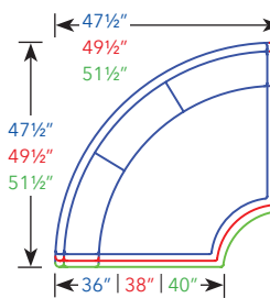
Curved Wedge 5510CP, 47 1/2" x 36" 6610CP, 49 1/2" x 38" 7710CP, 51 1/2" x 40"
