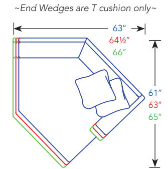
Right Facing End Wedge 5508R, W 68" x D 51" 6608R, W 70" x D 53" 7708R, W 72" x D 55"
