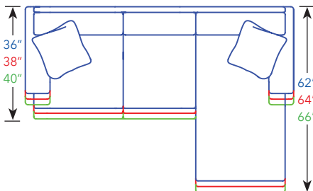
36" 38" 40" 62" 64" 66" Sofa/Chaise Combo, ISW 79" 5534-95 L/R 6634-95 L/R 7734-95 L/R
