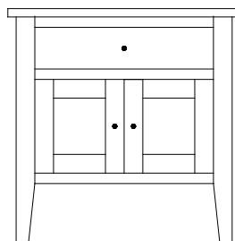
CS-1644 Night Stand 28"w 28"h 17½"d w/1 drawer, 2 doors
