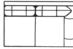
3575-1R RIGHT ARM LOVESEAT H36 W57 D38 INSIDE: H16 W47 D22 SEAT H: 20 ARM H: 22
